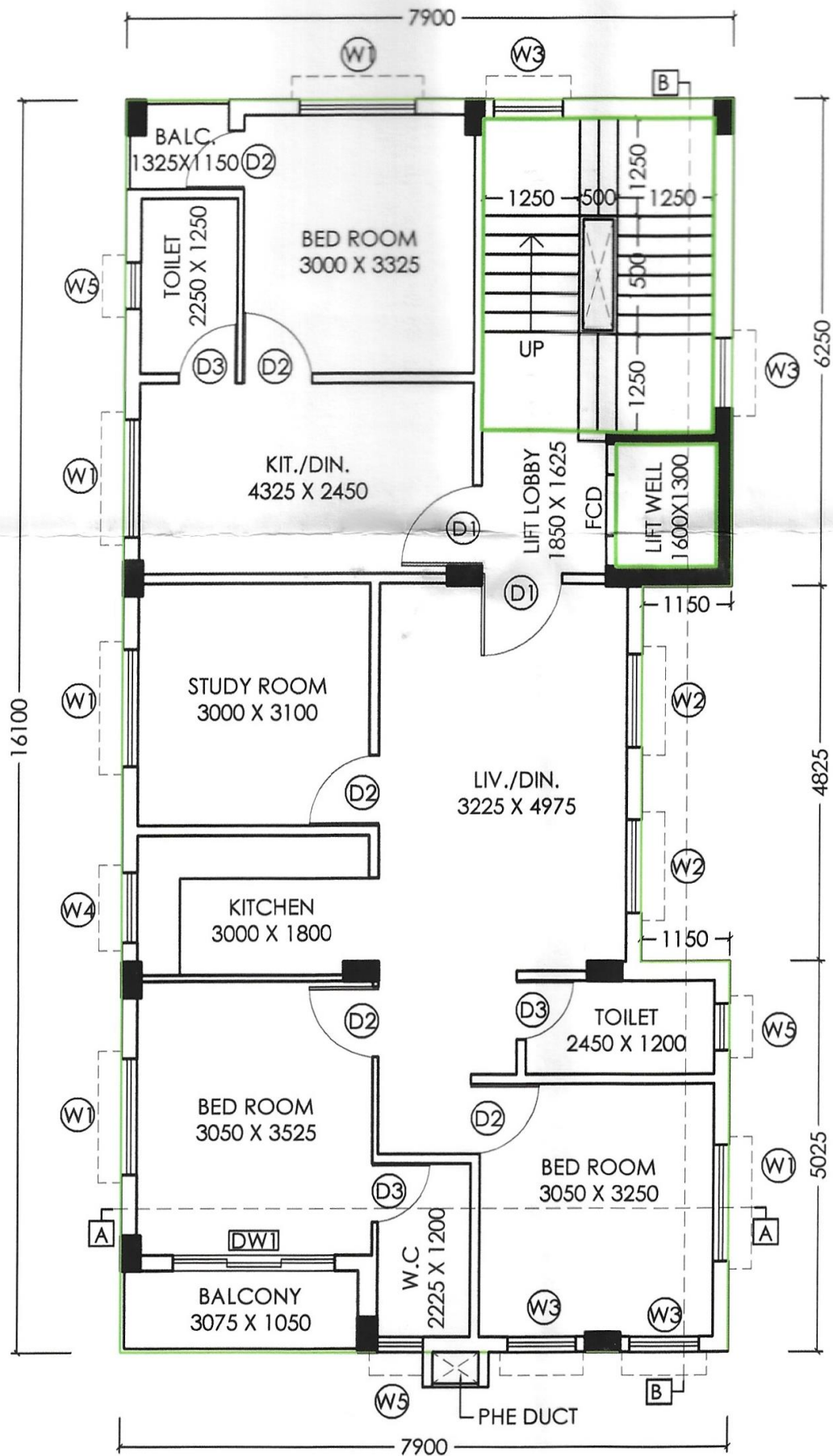
TYPICAL FLOOR PLAN (1ST. TO 4TH.) SCALE - 1:100
